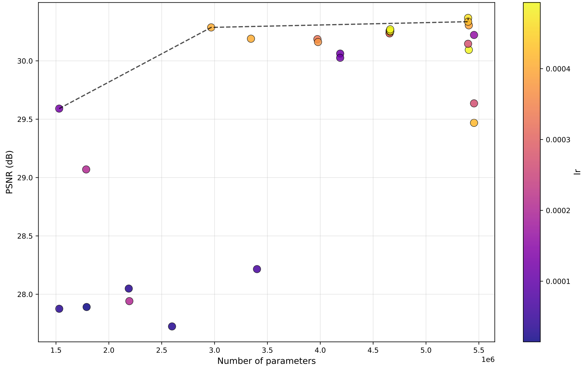
PSNR vs #Params — WaveletAttention — by l_r
